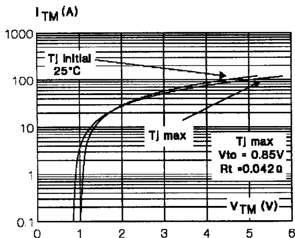
Fig.9 : On-state characteristics (maximum values).
