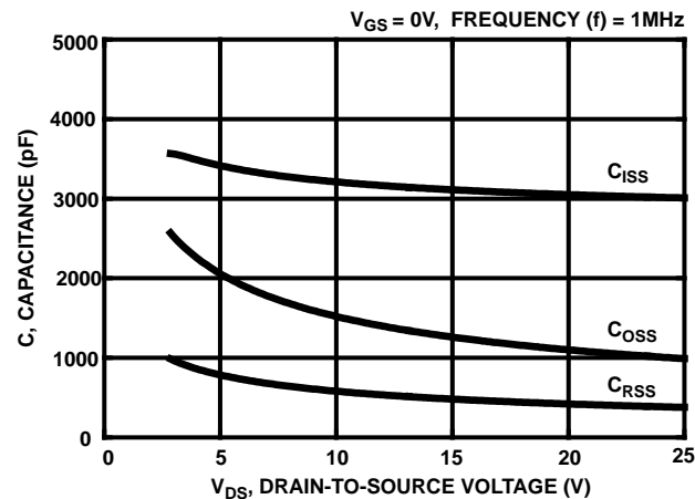
FIGURE 11. TYPICAL CAPACITANCE vs VOLTAGE
